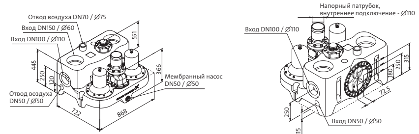
MULTILIFT MD
