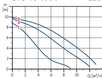
UPS 40-100 F 220
